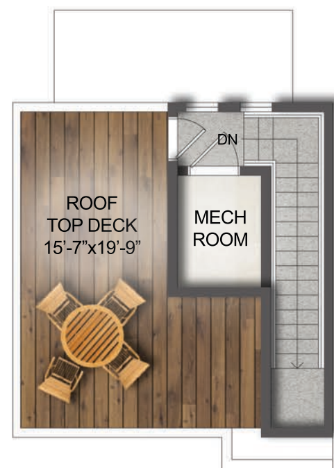
LEVEL 4 PLAN
